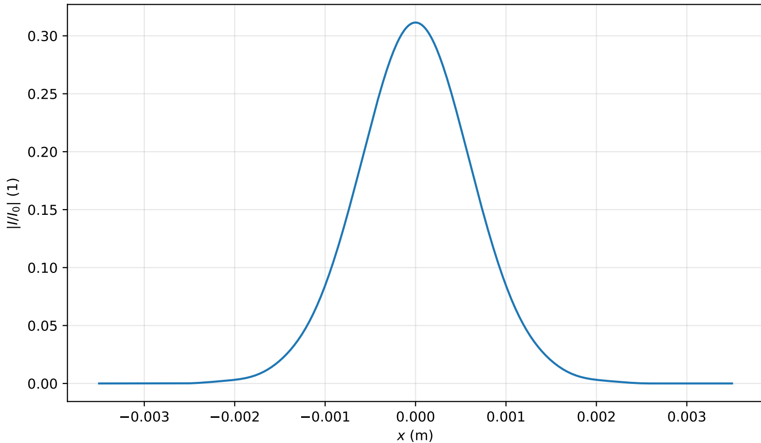
Intensity profile I(x, y = 0, z = 3.742m)/I_0 , P_{in}=0.3P_{cr} , artificial time
